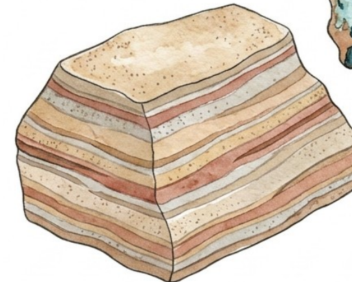
SANDSTONE (SEDIMENTARY)
